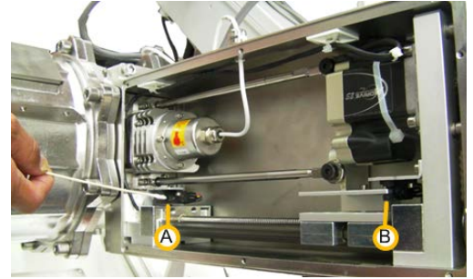
Figure 10-54: Generic Location of the DPM Opto-couplers (Generic View)
