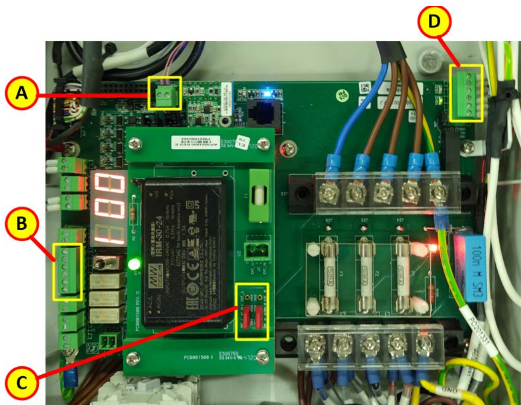
Figure 5-20: Connection Box LM Card I300+I500 (for RZ system without cleaner)
