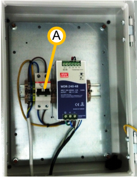
Figure 10-55: 48VDC Module Circuit Breaker
