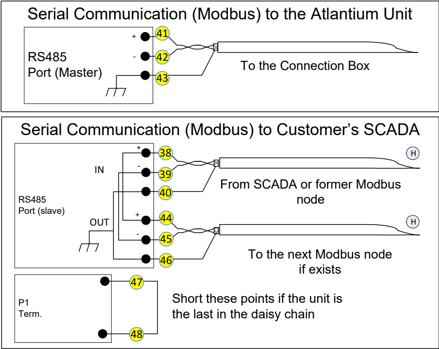
Figure 5-29: Serial Communication (Modbus) Connections
