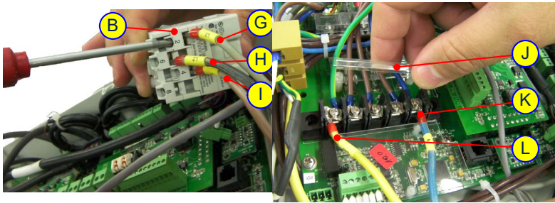
Figure 5-35: Replacing the Power Cable 4
