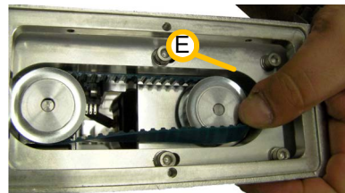
Figure 10-59: Inserting the Replacement Belt
