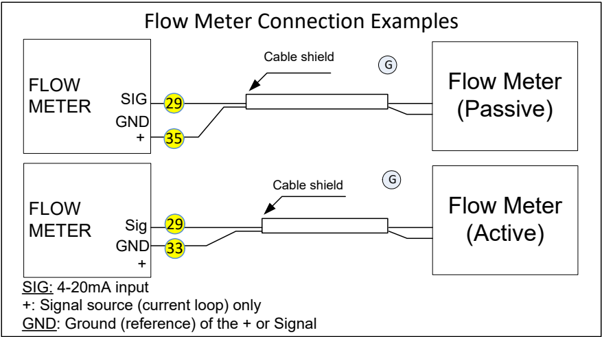
Figure 5-28: Flow Meter Connection Examples
