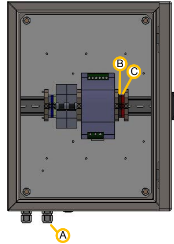
Figure 5-23: Connecting the 48VDC Cable
