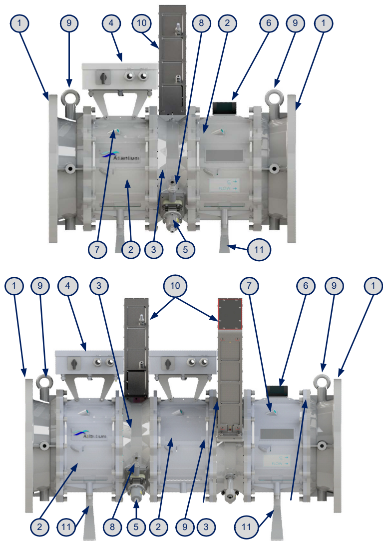
Figure 2-1: RZ300 unit, with DPM cleaner (see table below)
