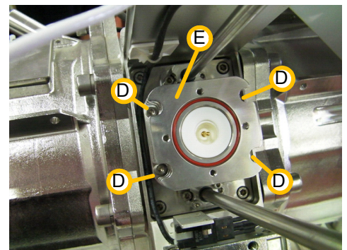
Figure 10-13: Remove the Lamp's Housing
