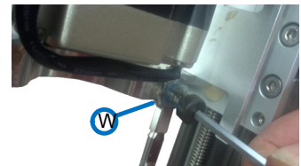
Figure 10-39: Installing the Plate and Wiper Assembly
