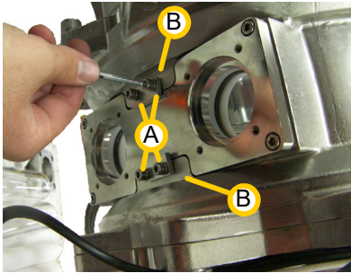
Figure 10-61: Unfastening the Brackets
