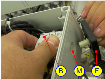
Figure 5-37: Replacing the Power Cable 6
