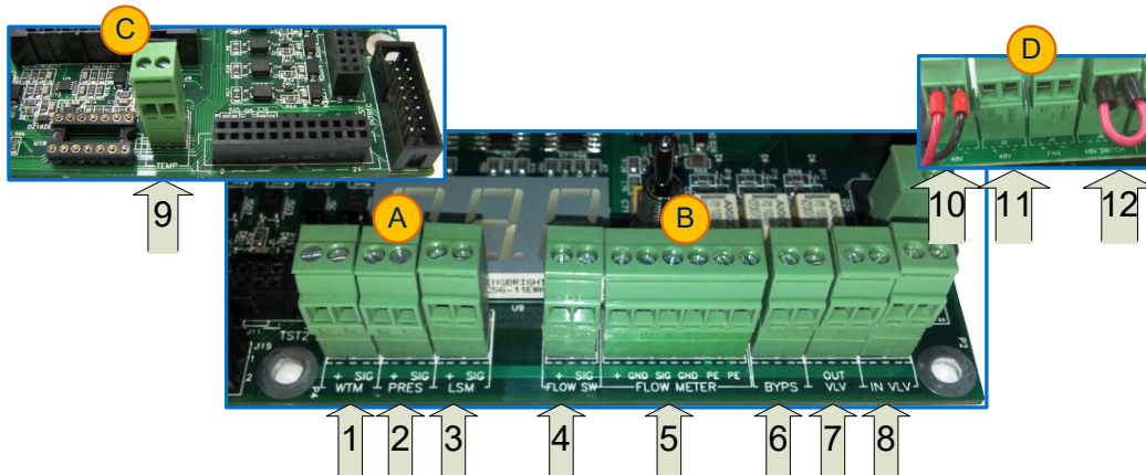
Figure 5-21: Connectors on Connection Box Card 1300+1400
