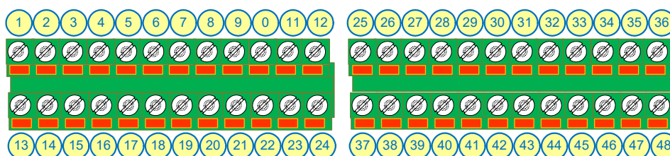
Figure 5-25: Control Module Terminal Connectors
