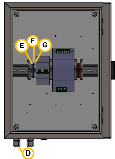
Figure 5-30: Connecting the Mains to the 48VDC Module
