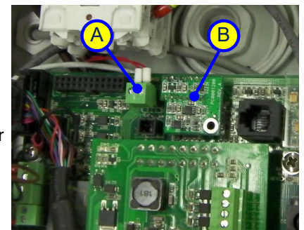
Figure 10-75: Location of the Temperature Sensor Connector (Generic)
