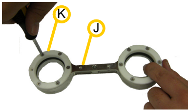
Figure 10-67: Opening the Wiper Assembly
