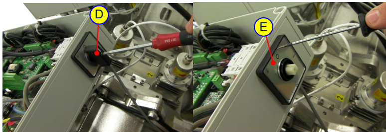
Figure 5-32: Replacing the Power Cable 1
