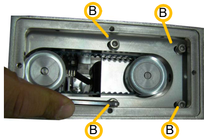
Figure 10-56: DPM Mechanism Top Screws
