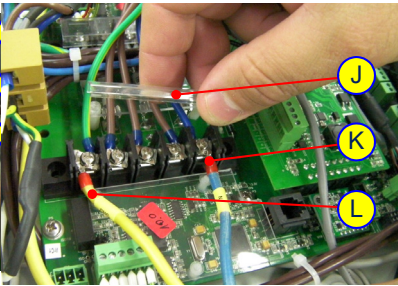
Figure 5-36: Replacing the Power Cable 5
