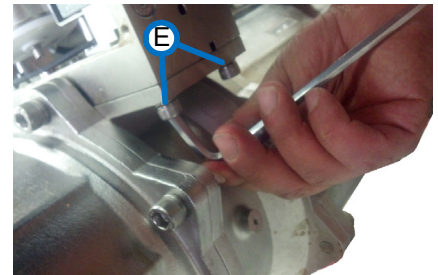
Figure 10-32: Unfastening the DPM Frame - Lower Bolts
