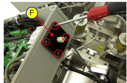
Figure 5-34: Replacing the Power Cable 3
