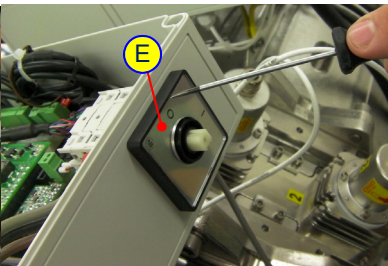
Figure 5-33: Replacing the Power Cable 2
