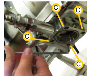
Figure 10-37: Removing the Quartz Sleeve's Holder on the Lower Side
