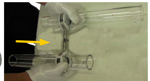
Figure 10-73: Placing the Wiper Assembly - View 2
