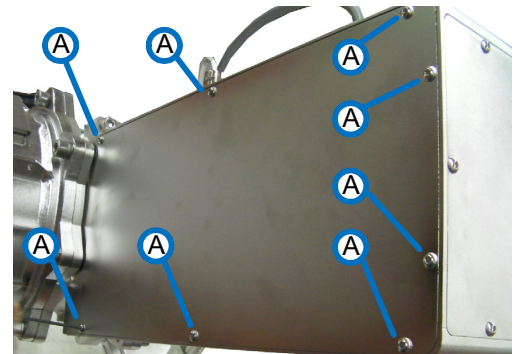
Figure 10-28: DPM Cover's 8 screws
