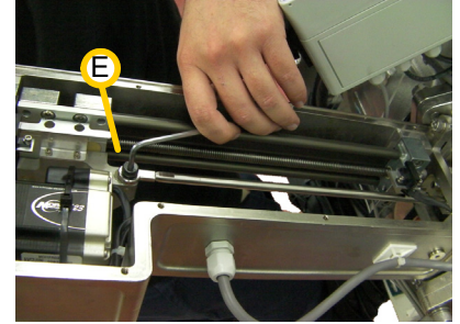
Figure 10-63: Unfastening the Wiper Assembly's Rod
