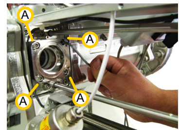
Figure 10-35: Removing the Quartz Sleeve's Holder
