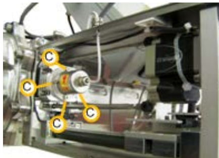
Figure 10-10: Removing the Lamp's Connector Assembly
