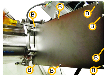
Figure 10-12: DPM Cover's eight screws
