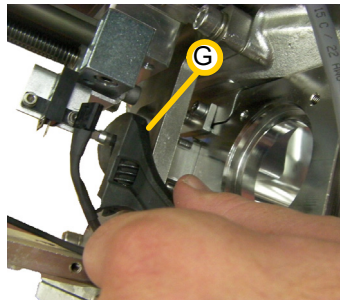
Figure 10-65: Gripping the Wiper Assembly's Rod
