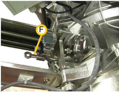
Figure 10-64: Wiper Assembly's Rod is Pushed All the Way Down
