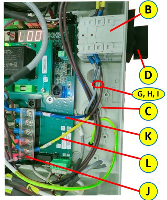
Figure 5-31: Power cable connections to connection box
