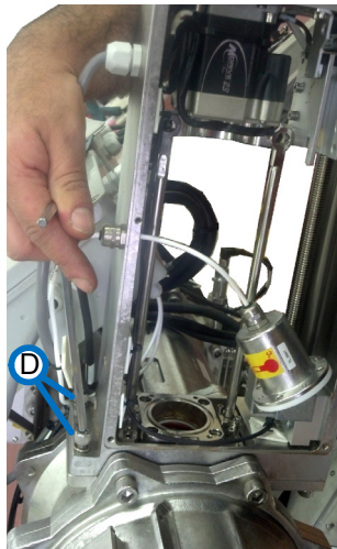
Figure 10-31: Unfastening the DPM Frame - Upper Bolts
