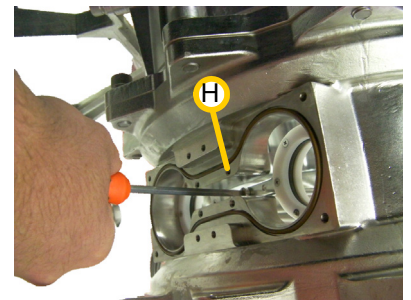
Figure 10-66: Unfastening the Central Bolt of the Wiper Assembly
