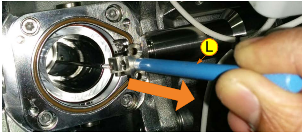
Figure 10-20: Removing the Wave Guide (Generic View)
