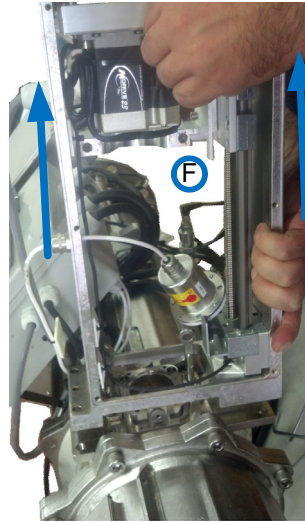
Figure 10-33: Removing the DPM Frame
