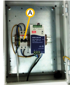
Figure 10-11: 48VDC Module Circuit Breaker
