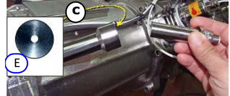
Figure 10-51: Replacing the Sensors 3 (Generic View)
