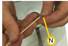
Figure 10-70: Applying Loctite to the Screws
