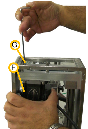
Figure 10-60: Tightening the screws (Generic View)
