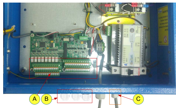
Figure 5-24: Control Module Interior Generic
