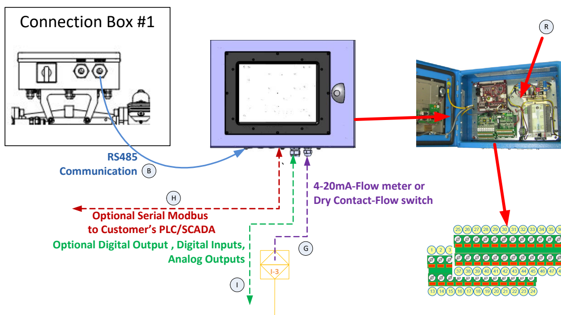
Figure 5-26: Digital and Analog Input and Output Connections-Schematic Diagram
