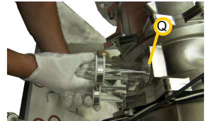
Figure 10-74: Insert Quartz Tubes
